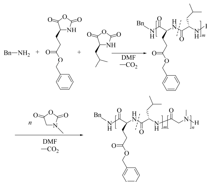
Scheme 1 Synthesis of poly(BLG- r -Leu) and poly(BLG- r -Leu)- b -polySar
