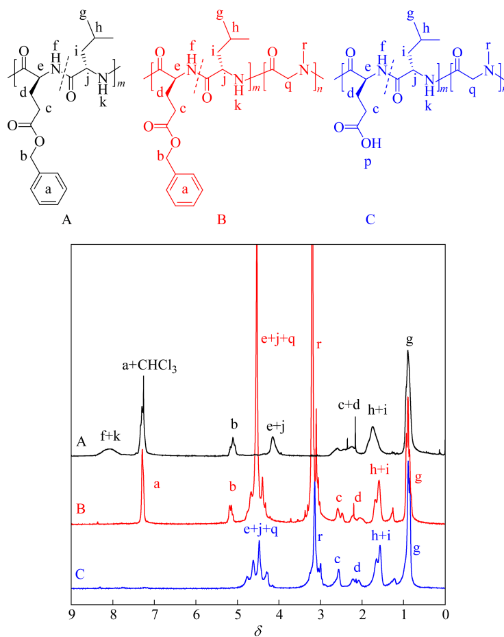
Fig. 6 ^1\text{H} -NMR spectra of poly(BLG- r -Leu) in \text{CDCl}_3/\text{CF}_3\text{COOH} (2:1) mixture (A), poly(BLG- r -Leu)- b -polySar in \text{CF}_3\text{COOD} (B) and poly(Glu- r -Leu)- b -polySar in \text{CF}_3\text{COOD} (C)
