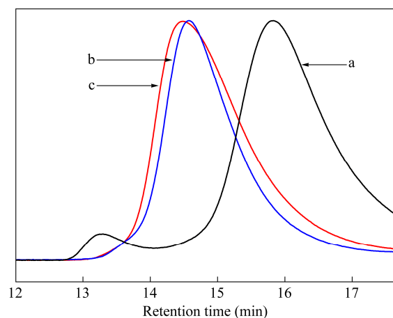
Fig. 7 SEC profiles of PBL-70 (a), PBLS-200 (b) and PBLS-400 (c)
