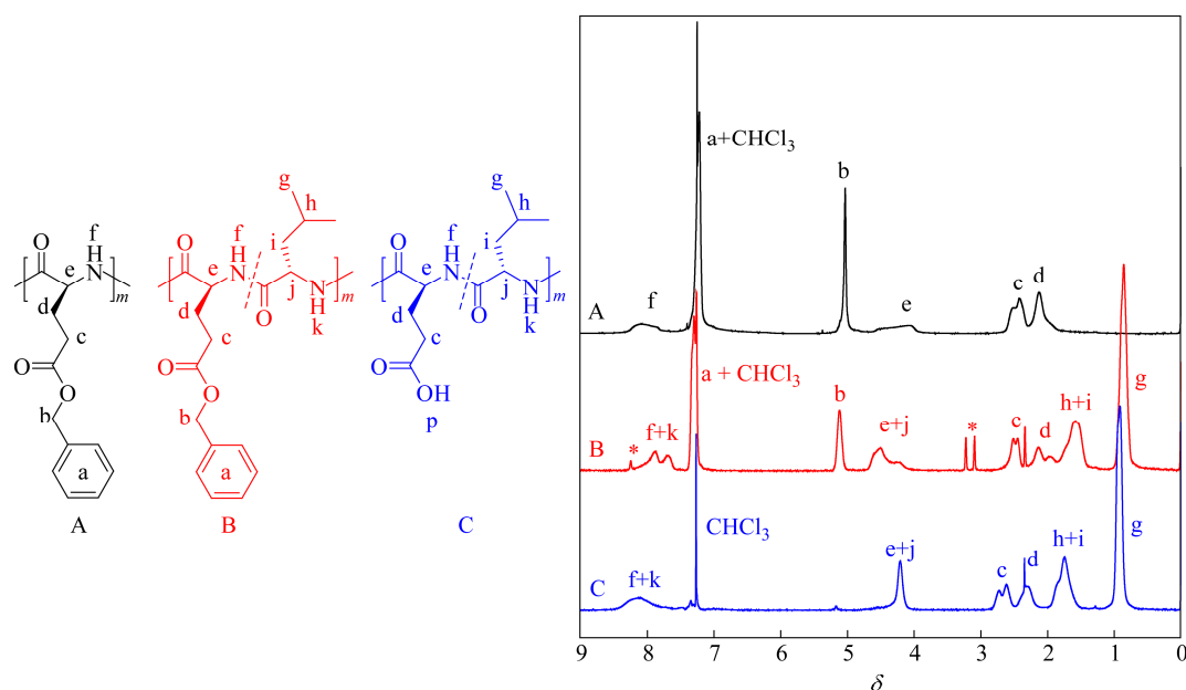
Fig. 1 ^1\text{H} -NMR spectra of polyBLG (A), poly(BLG- r -Leu) (B) and poly(Glu- r -Leu) (C) (* DMF. The solvent is \text{CDCl}_3/\text{CF}_3\text{COOH} (2:1) mixture.)
